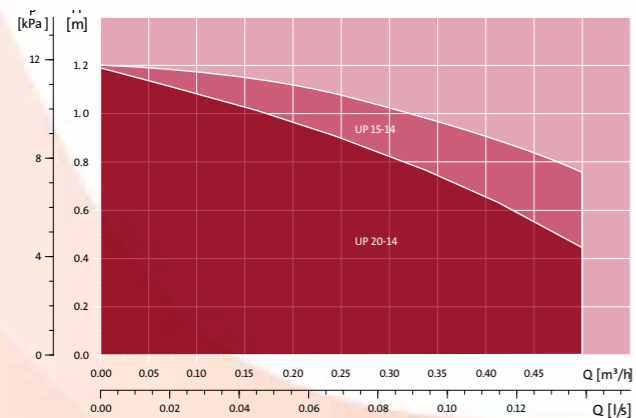
Performance curves for the COMFORT range.
